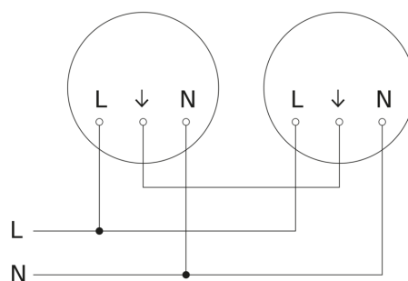
Master/master interconnection circuit diagram
